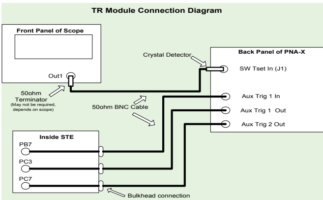
Typical TR Module Test Setup
