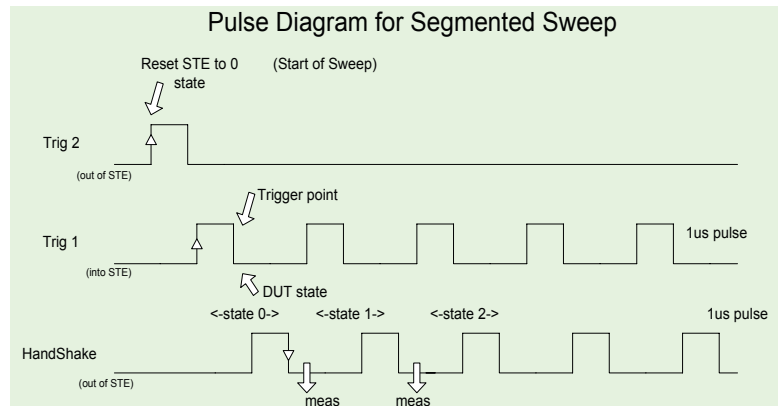
Typical Measurements Timing Diagram
